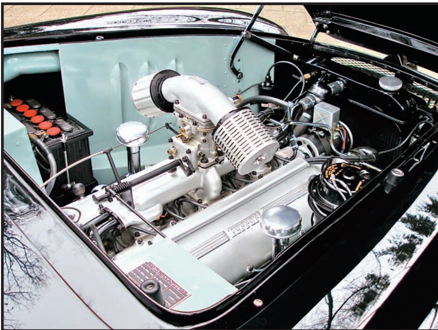
Above: "The 212 Inter carried a single Weber 36 DCF carburetor, and it put out about 150 bhp at 6500 rpm. This power gave the 212, with its five speed box, a top speed of 182 kmh."
